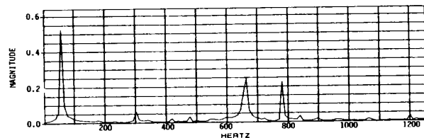
FIG.13. VOLTAGE AT 25 KV BUS WITH FILTERS CONNECTED.
