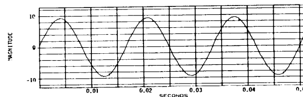
FIG.13. VOLTAGE AT 25 KV BUS WITH FILTERS CONNECTED.
