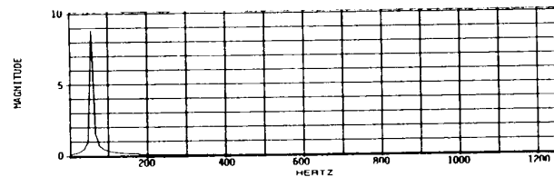
FIG.12. INCOMING LINE CURRENT TO 25 KV BUS.
