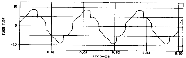
FIG. 11. CONVERTER TRANSFORMER SECONDARY CURRENT IN 12-PULSE SYSTEM
