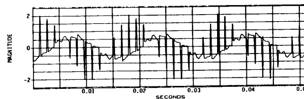
FIG.14. TOTAL CURRENT IN HARMONIC FILTERS CONNECTED TO 25 KV BUS.
